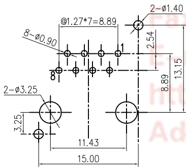
RECOMMEND PCB LAYOUT (TOLERANCE=±0.05)
