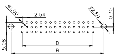
RECOMMEND PCB LAYOUT(FOR MALE) THICKNESS=1.6±0.10mm
