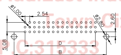
RECOMMEND PCB LAYOUT(FOR FEMALE) THICKNESS=1.6±0.10mm
