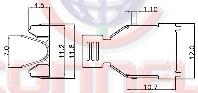
Upper shell
