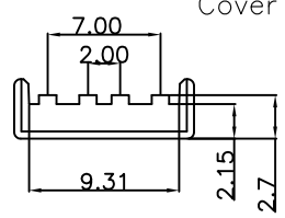
Cover
