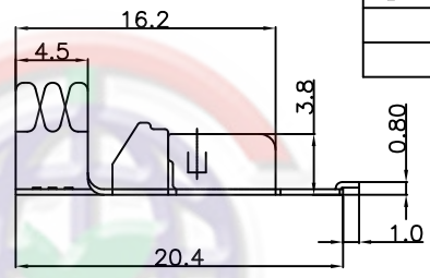
Upper shell
