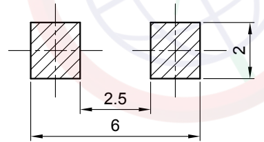
Recommend PCB layout Tolerance±0.05
