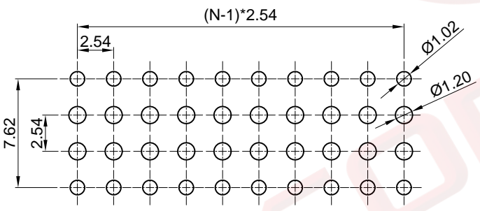
Recommend PCB layout (Tolerance: \pm 0.05 )
