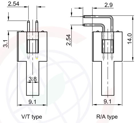
Dimension
